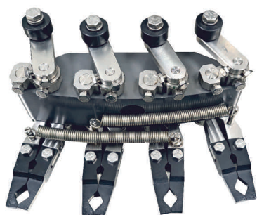
Vial Finger Assembly-1
