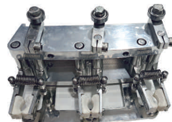
Vial Finger Assembly-2
